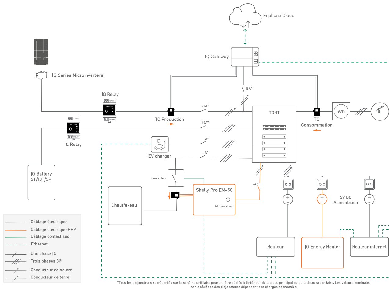
Illustration 1: Configuration monophasée
